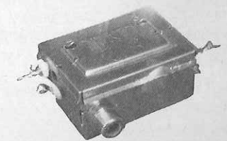
E & P video modulator
