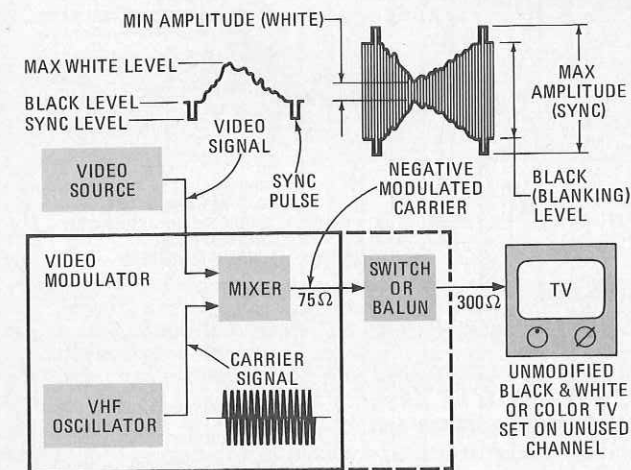
FIG. 1—BLOCK DIAGRAM OF VIDEO MODULATOR.
